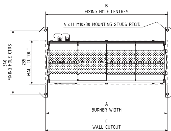
FDB06 Burner and rear mounted combustion air fan
